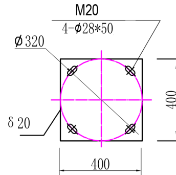
Base plate details
