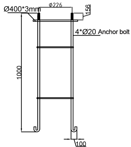
Anchor bolt details
